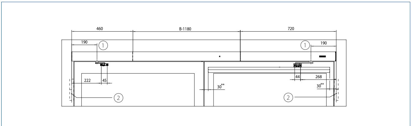
B = Hinge clearance | ** = Recommended size for installation of the GC 335 and GC 338 sensor strip | 1 = Hinge clearance | 2 = Dimensional reference centre of hinge
