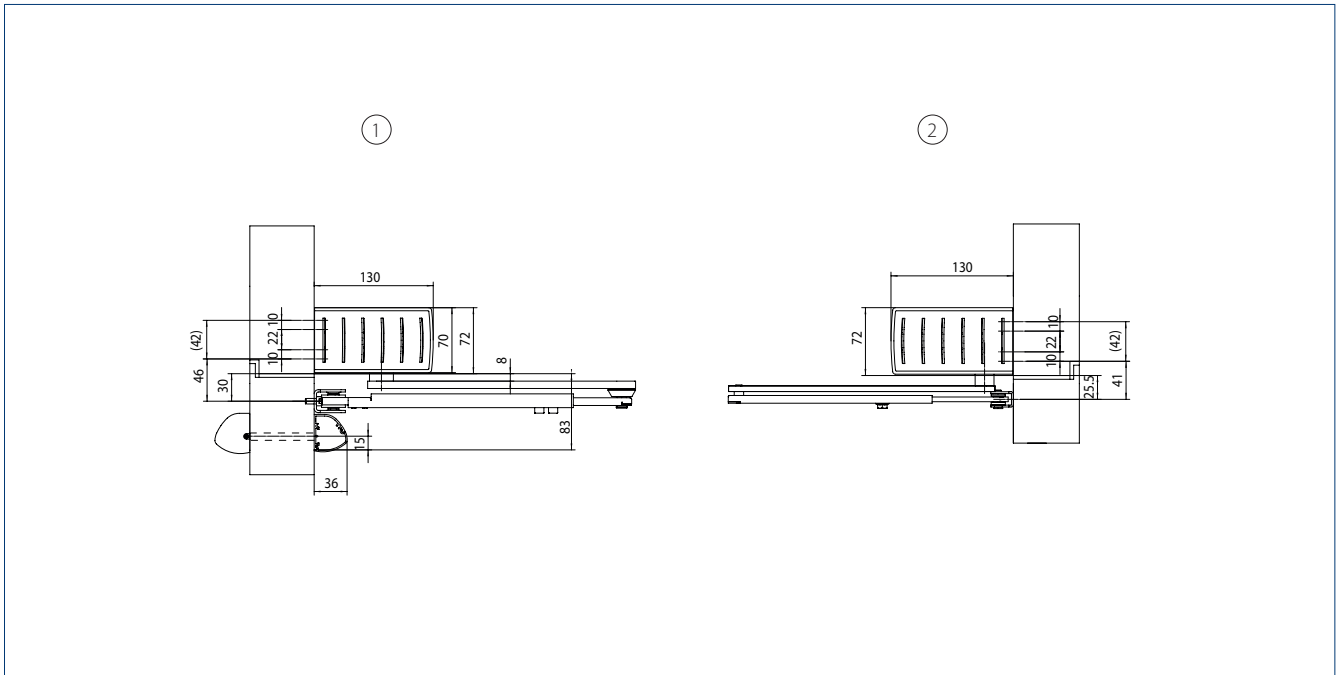
1 = Powerturn with link arm and GC 338 sensor strip | 2 = TS 4000 door closer with link arm
