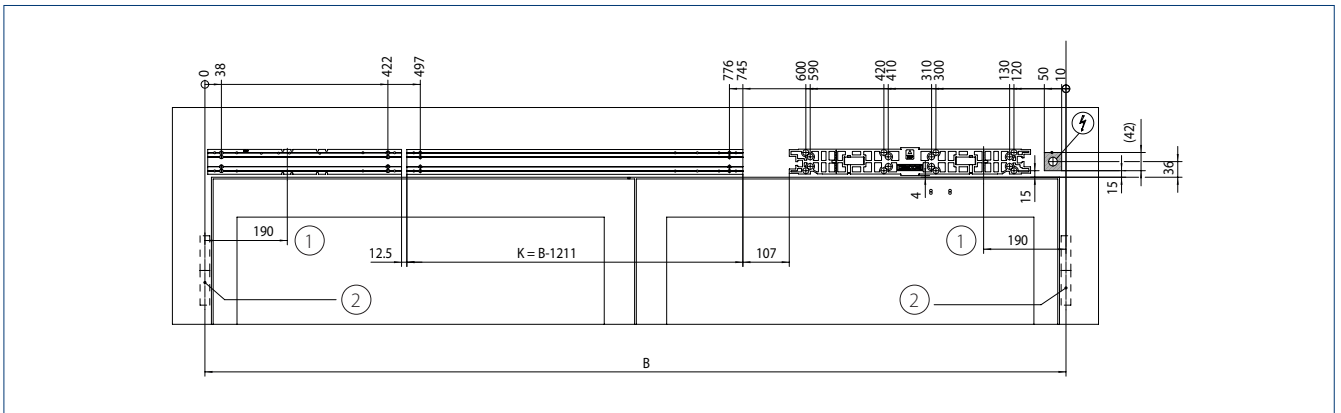
K = Position of the intermediate base plate | B = Hinge clearance | 1 = Hinge clearance | 2 = Dimensional reference centre of hinge
